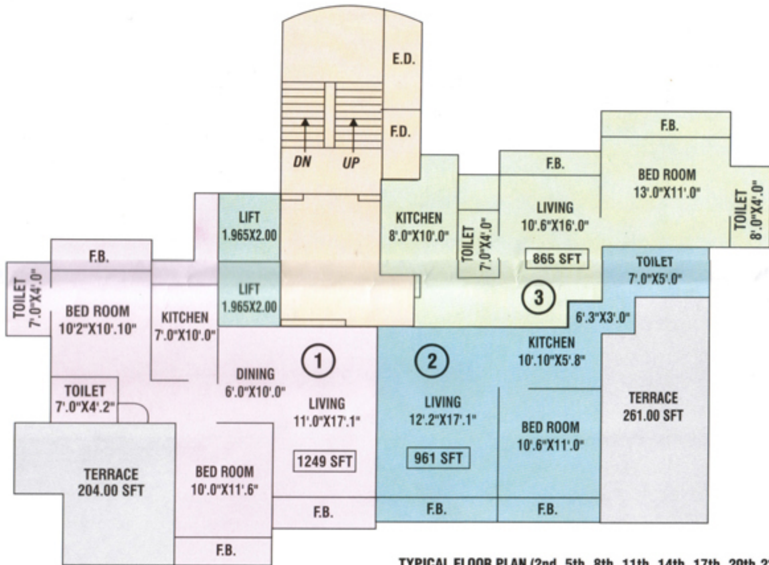
TYPICAL FLOOR PLAN (2nd, 5th, 8th, 11th, 14th, 17th, 20th, 23rd & 26th Floor)
