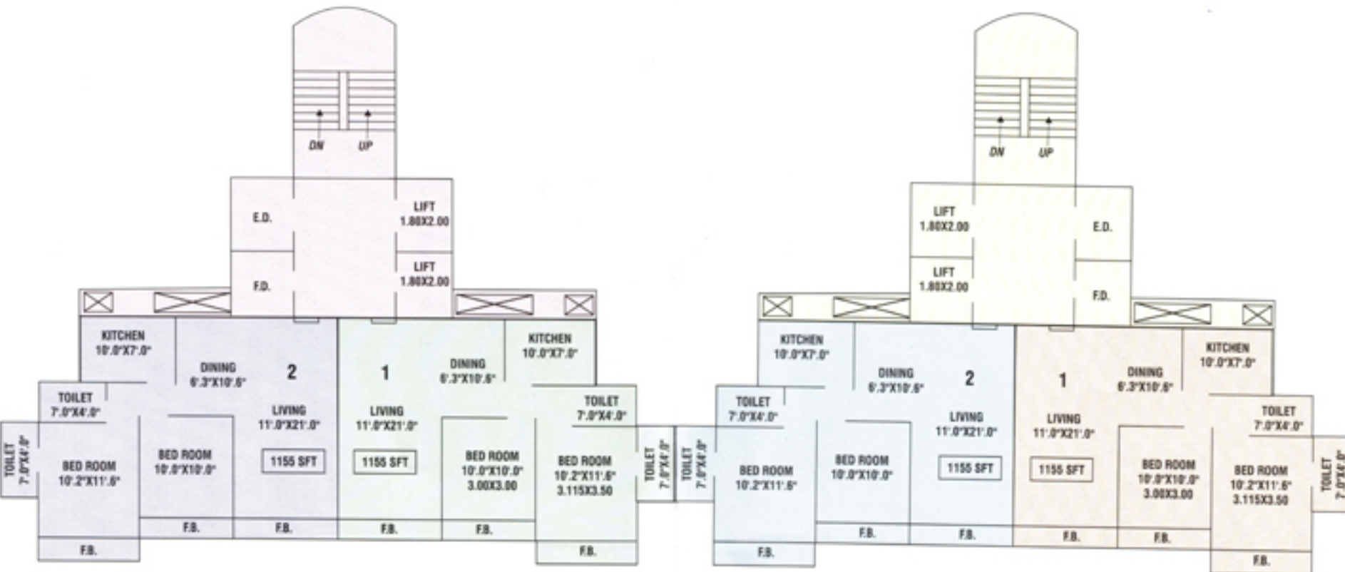
TYPICAL FLOOR PLAN (2nd to 26th Floor)
