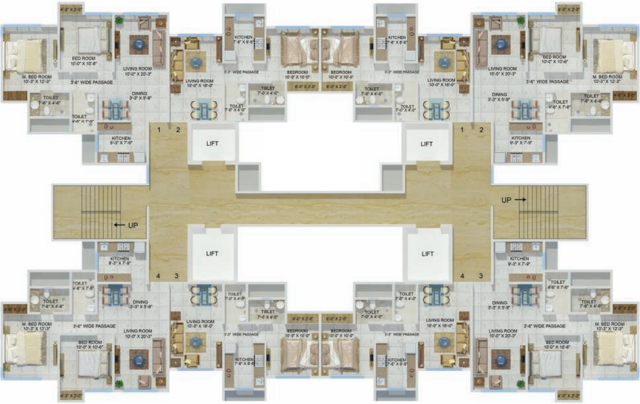
Typical Floor Plan | B Wing
